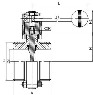
手动螺纹蝶阀 Manual threaded butterfly valve NO.1101010
