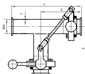
三通蝶阀(右开型) Three-way butterfly valve ( Right open type )
