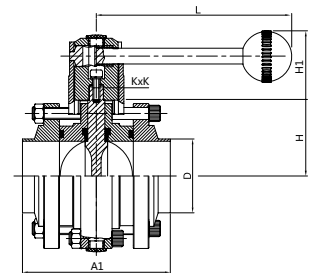
三片式 Three-piece butterfly valve
