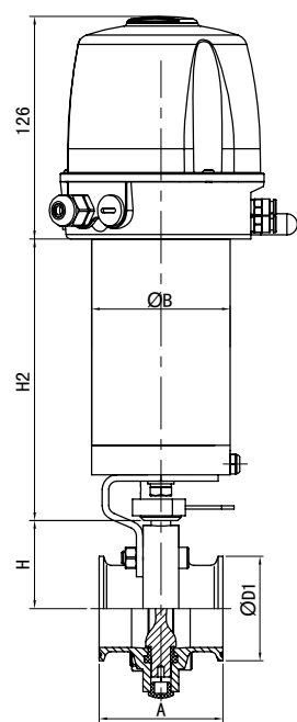
带智能头不锈钢气动快装蝶阀 SS pneumatic clamped butterfly valve with C-top NO.1101006
