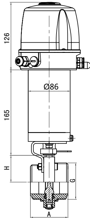
带智能头不锈钢气动螺纹蝶阀 SS Pneumatic threaded butterfly valve with C-top NO.1101015
