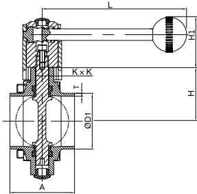
手动焊接蝶阀 Manual welded butterfly valve NO.1101001
