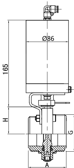
不锈钢气动螺纹蝶阀 SS pneumatic threaded butterfly valve NO.1101014
