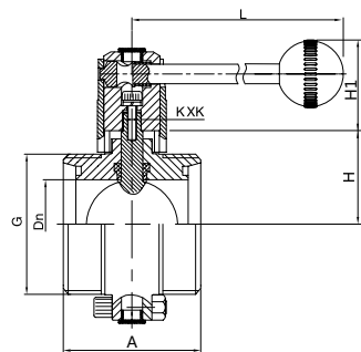
手动螺纹蝶阀 Manual threaded butterfly valve NO.1101007
