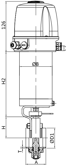
带智能头不锈钢气动焊接蝶阀 SS pneumatic welded butterfly valve with C-top NO.1101003
