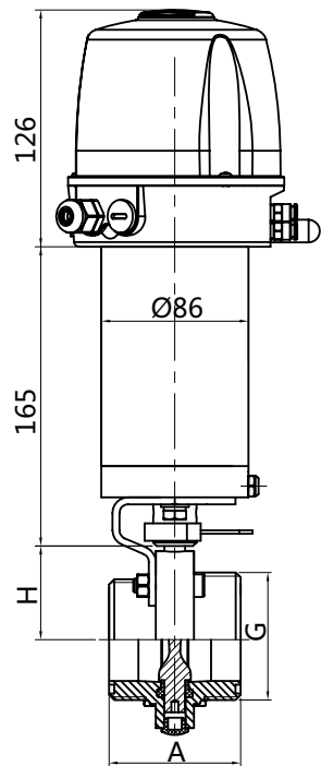
带智能头不锈钢气动螺纹蝶阀 SS pneumatic threaded butterfly valve with C-top NO.1101012
