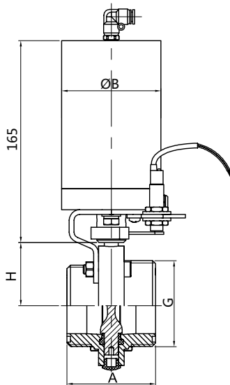
不锈钢气动螺纹蝶阀 SS pneumatic threaded butterfly valve NO.1101011
