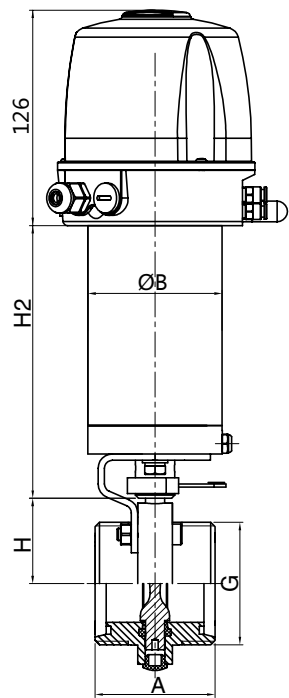
带智能头不锈钢气动螺纹蝶阀 SS pneumatic threaded butterfly valve with C-top NO.1101009
