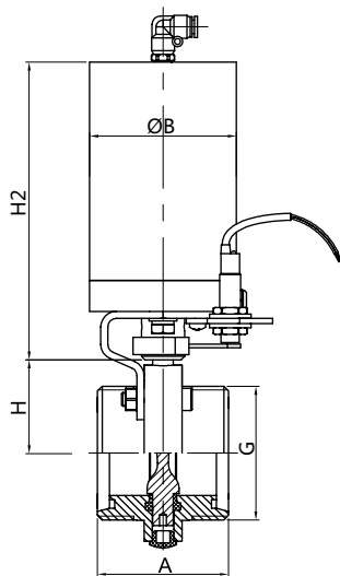
不锈钢气动螺纹蝶阀 SS pneumatic threaded butterfly valve NO.1101008
