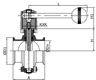
手动快装蝶阀 Manual clamped butterfly valve NO.1101004
