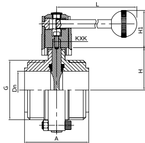
手动螺纹蝶阀 Manual threaded butterfly valve NO.1101013
