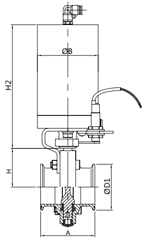
不锈钢气动快装蝶阀 SS pneumatic clamped butterfly valve NO.1101005
