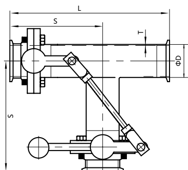
三通蝶阀(左开型) Three-way butterfly valve ( Left open type )
