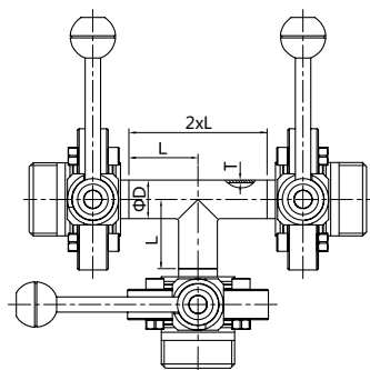
三通蝶阀 Three-way butterfly valve
