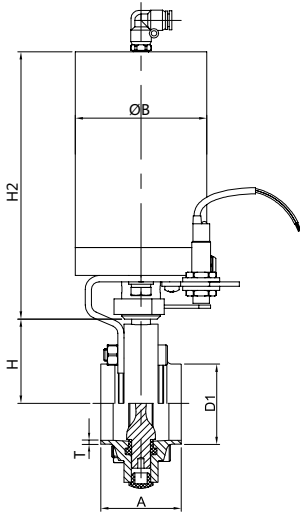
不锈钢气动焊接蝶阀 SS pneumatic welded butterfly valve NO.1101002
